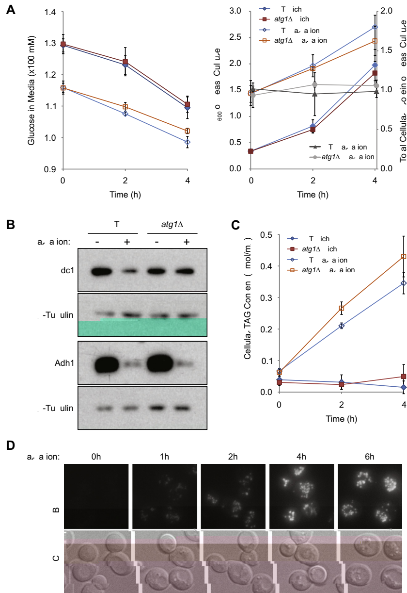
Fig. 1. Under nitrogen starvation, yeast cells continue to consume glucose, downregulate fermentation enzymes and increase storage lipid synthesis. (A) Glucose consumption and growth of yeast cells in rich medium and nitrogen starvation medium. Concentration of glucose in the media, optical density (OD 600 ) and total cellular protein of the culture were measured for wild type and atg1Δ yeast cells. For samples in rich medium, time zero is when OD 600 reached approximately 0.35. For starved samples, time zero is when in rich medium, slightly more glucose was added to shift all data points up. For total cellular protein, the average of each repeat was normalized as 1. Error bar, standard deviation from three independent experiments. (B) Expression of key enzymes involved in fermentation. The indicated enzymes were chromosomally tagged with 3xHA at the carboxyl termini. Protein samples were collected from wild type and atg1Δ yeast cells at mid-log phase or after 4 h of starvation, and analyzed by immunoblotting. The experiment was repeated three times and representative images are shown. \alpha -tubulin was used as a loading control. (C) Cellular TAG content of yeast cells in rich medium and in nitrogen starvation medium. Cellular TAG content (expressed as TAG/total protein) was measured for wild type and atg1Δ yeast cells. Data are presented as in panel A. (D) BODIPY staining of LDs. At time zero, mid-log phase wild type yeast cells were shifted to nitrogen starvation medium. At the indicated time points, cells were stained with BODIPY and imaged by fluorescent microscopy. The experiment was repeated three times and representative images are shown. For the BODIPY channel, a maximum intensity projection of a Z-stack is presented. DIC: differential interference contrast. Note that our imaging parameters were optimized for starved cells, which resulted in LDs in growing cells being almost invisible.
