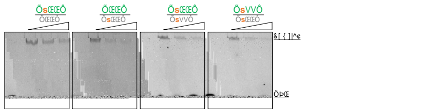
FIGURE 4 DNA PT modification at the GTTC side. (a) HPLC traces showing PT reaction with substrate DNA containing one PT modification. Substrate 1 contained a dGsA modification. Substrate 2 contained a dGsT modification. PT modification on the opposite side was then analyzed using HPLC/MS. For example, for substrate 1, dGsT was analyzed. (b) EMSA analysis of DndCDE binding to ds DNA with PT modification at one strand. Substrate DNA fluorescence is indicated by green color. Cold DNA is indicated with gray color. Ten- or 20-fold more unlabeled cold DNA was used for the experiments. (c) CD spectra of DndCDE protein binding to DNA with PT modification at one of the ds strands [Colour figure can be viewed at wileyonlinelibrary.com ]
