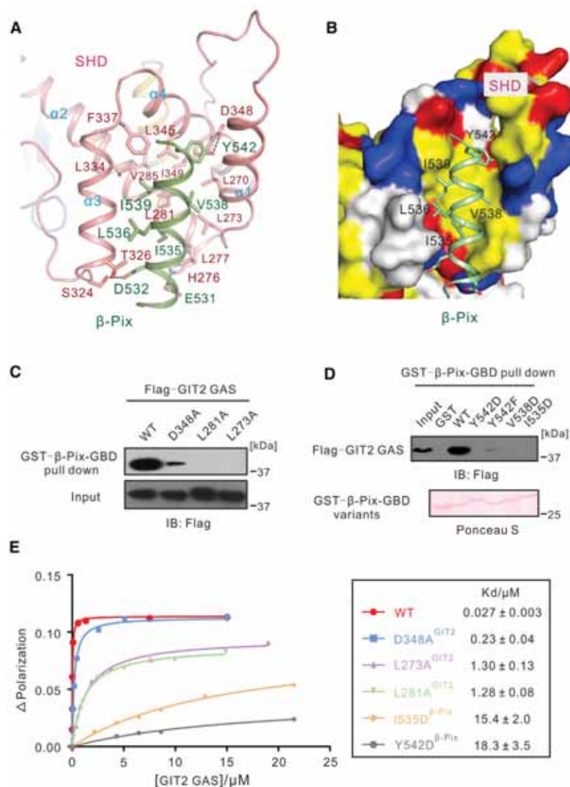
FIGURE 2. Molecular structure of GIT2/ \beta -Pix interface
